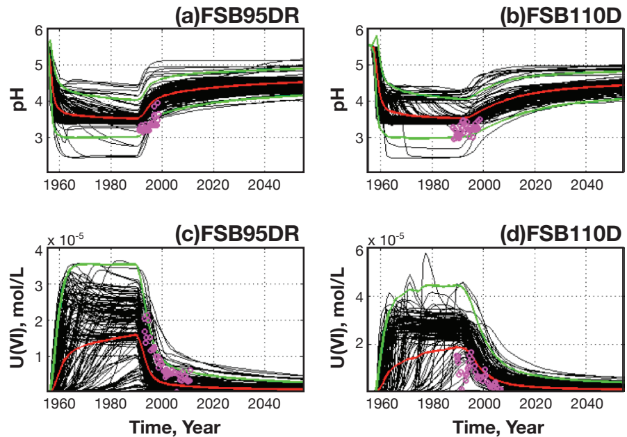
Figure 3 shows the Monte Carlo simulation result, which compares measured and simulated breakthrough curves of pH and the U(VI) at the two observation wells for pH and uranium concentrations (the field data were obtained from the ASCEM data management database). The observed breakthrough curves are fairly close to the predicted mean breakthrough curves and within the confidence bounds (mean \pm 2 standard deviations) except for some scattered observation points, which provides confidence in the validity of the model and simulations. The simulation results illustrate (Fig. 3a and 3b) that during the basin operations (1955-1988), pH values
