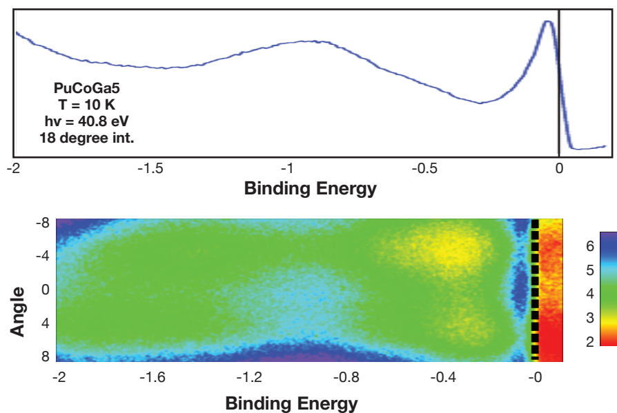
Figure 3. PES and ARPES data for \text{PuCoGa}_5 at a photon energy of 40.8 eV.
